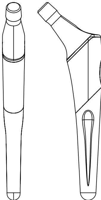
SIZE 8 LARGE TRUNNION
